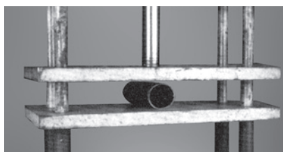
Epoxy Fiberglass conduit will flex back to almost its original shape after crushing.
